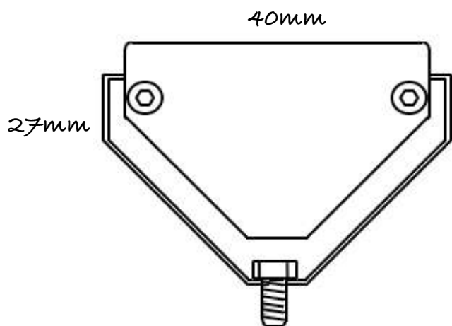
Front view of SS bracket for mounting directly behind - no swivel
