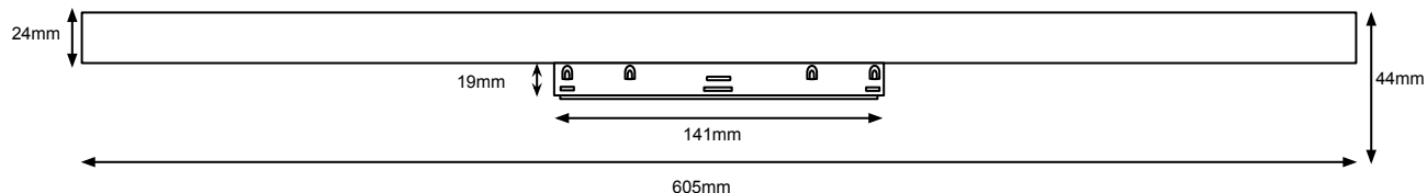
Ambient Light Side View: (20W)
