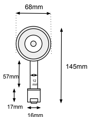
Fixed Spot Front View(30W):
