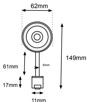
Variable Spot Front View (15W)
