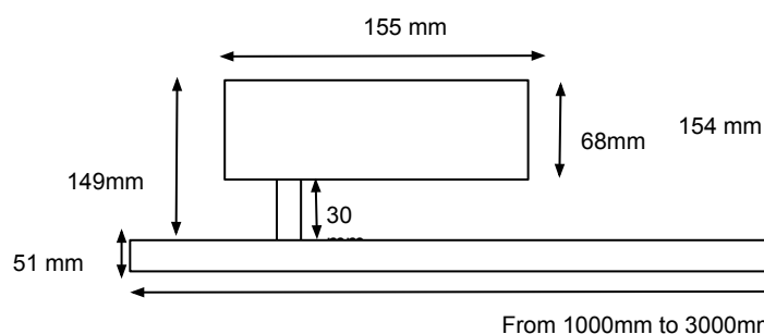
Fixed Spot On Track
