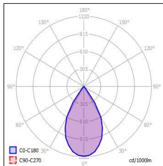
Variable Spot 15W 60°
