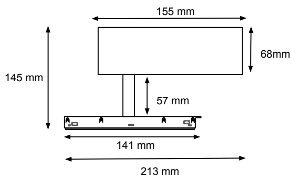
Fixed Spot Side View(30W):
