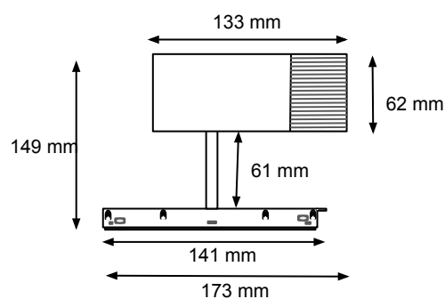
Variable Spot Side View (15W)
